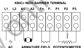
FIGURE 11. CONNECTION METHODS
