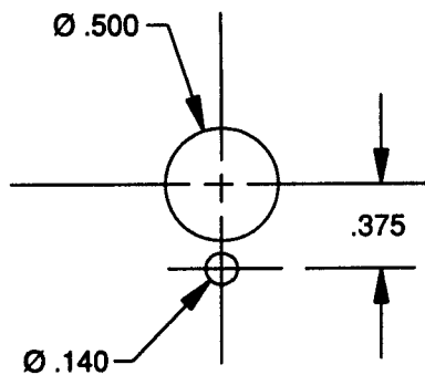
PANEL DRILLING
