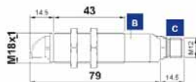
RECEIVER
