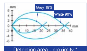
Detection area - proximity *
