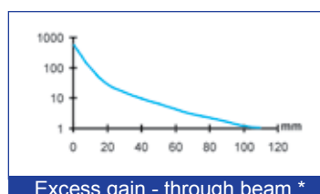
Excess gain - through beam *
