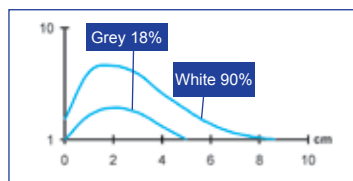
Excess gain - radial
