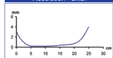
Resolution - radial
