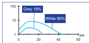
Excess gain - radial
