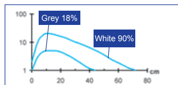
Excess gain - axial
