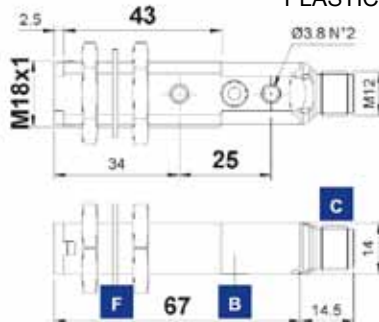
PLASTIC HOUSING
