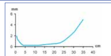
Resolution - axial
