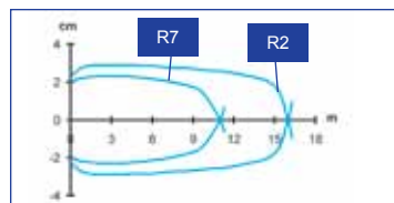
Detection area - axial
