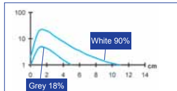
Excess gain - axial
