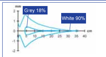
Detection area - axial
