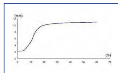
Resolution - axial
