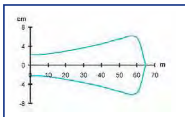
Detection area - axial
