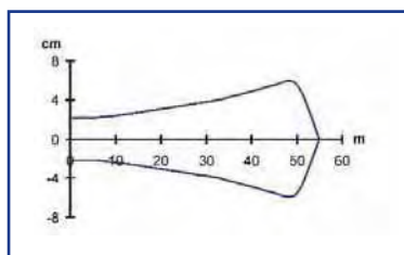
Detection area - radial
