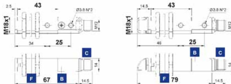
METAL HOUSING
