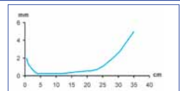
Resolution - axial
