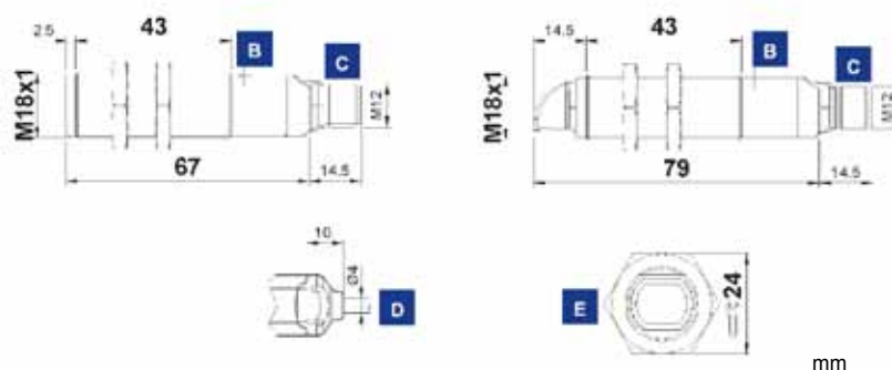
METAL HOUSING
