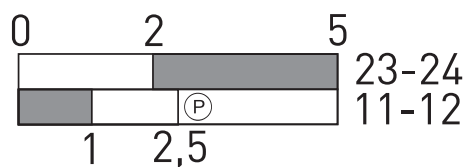
Switching diagram
