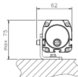
MOUNTING B
