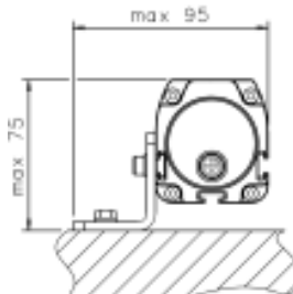
MOUNTING A
