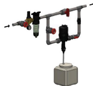
Bypass-Installation
