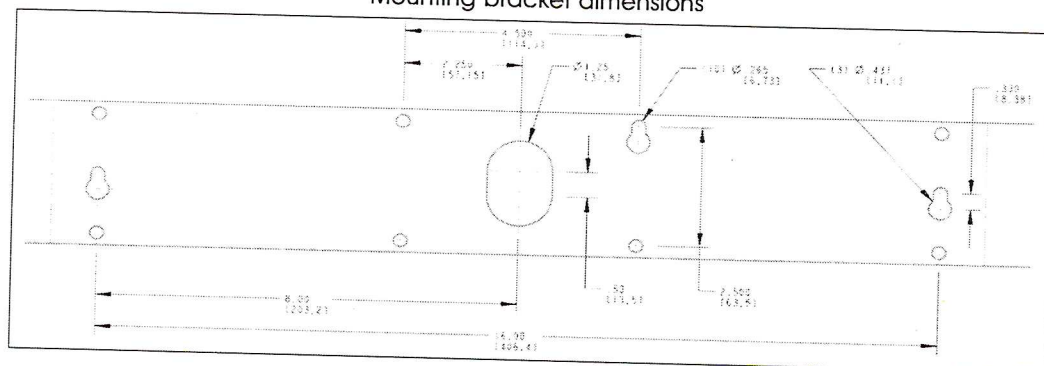
Mounting bracket dimensions
