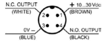
M12 CONNECTOR
