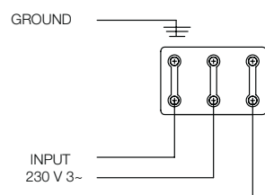
Connection at 230 V
