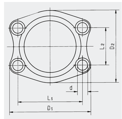
Flange according to SAE-standard
