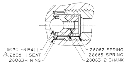
OUTLET CHECK VALVE
