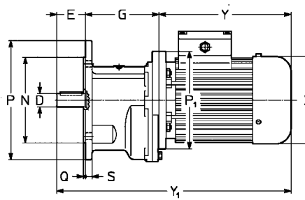
Standard design 1) Mounting position B5, V1, V3
