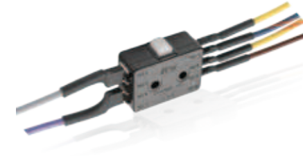
A Form CC DPDT (double pole double throw) mechanical switch with silver-plated contacts.
