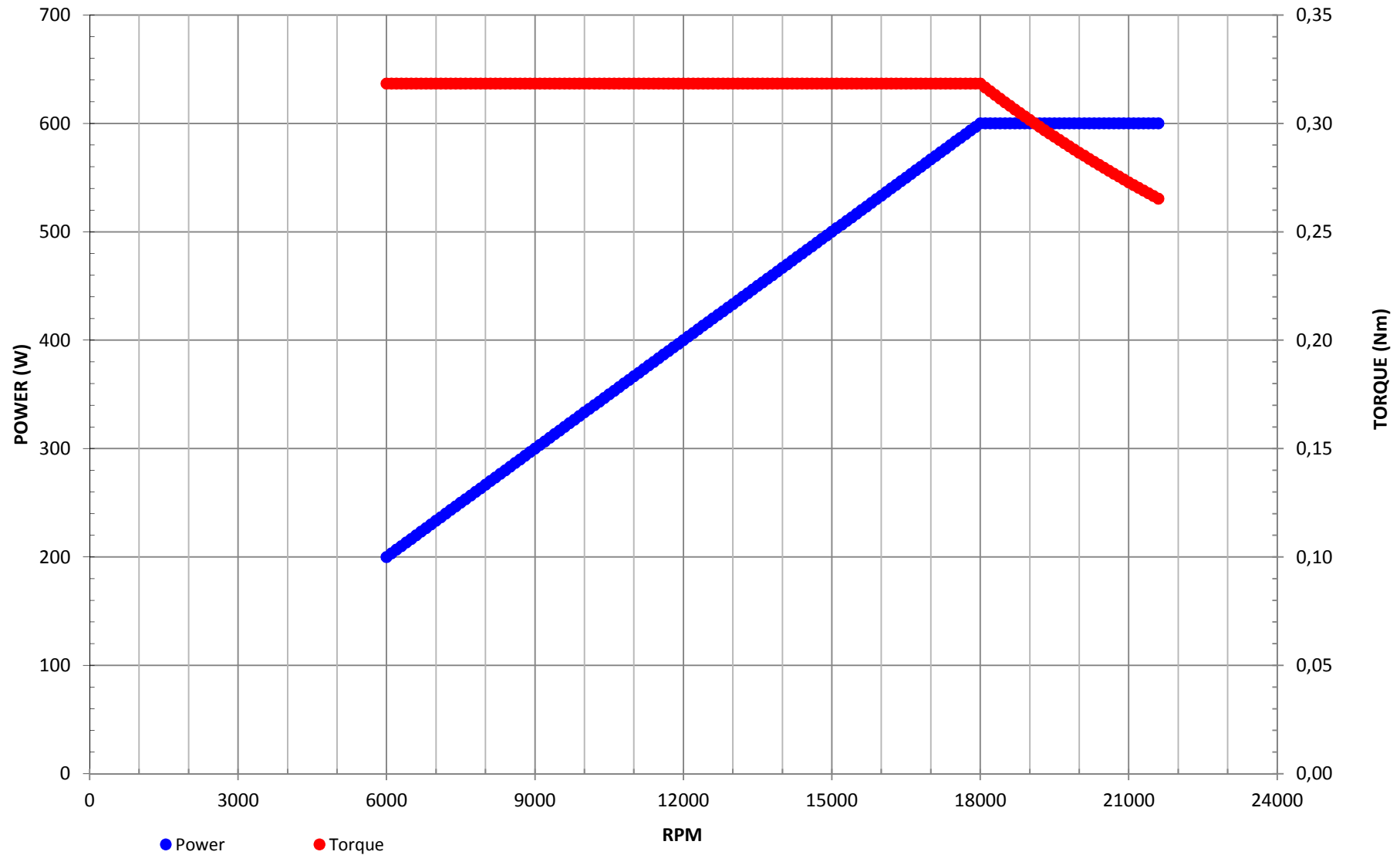
Torque & Power Curve TeknoMotor C35-C-SB-P-ER16-0.6KW-18000- 21600RPM
