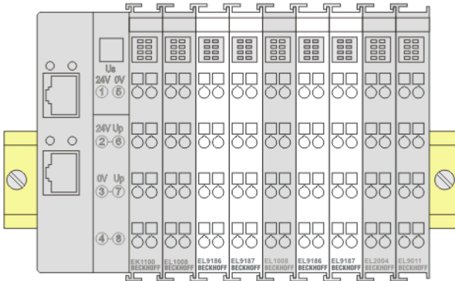
Fig. 59: Correct configuration
