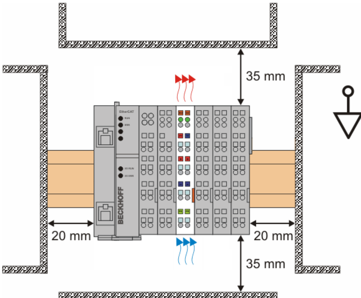
Fig. 57: Recommended distances for standard installation position
