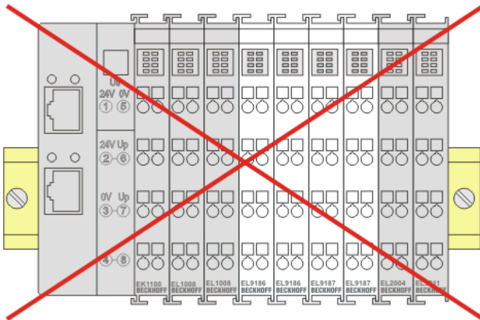
Fig. 60: Incorrect configuration
