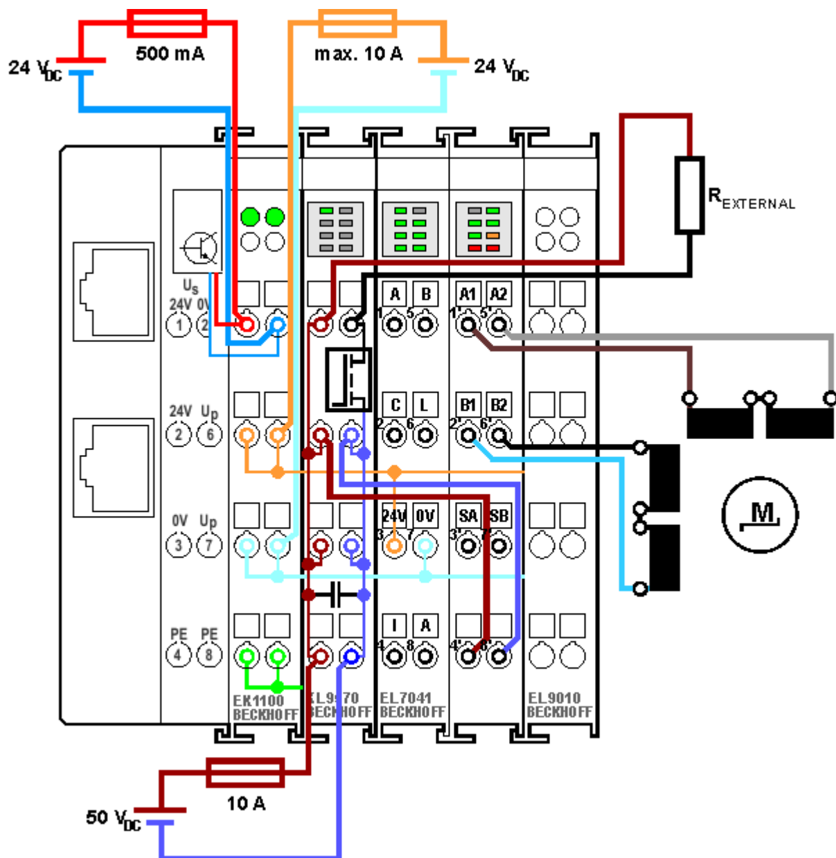
Fig. 42: Application example EL9570
