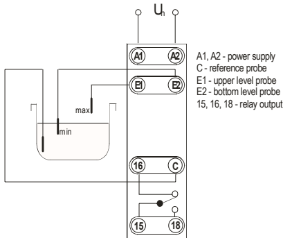
Connections for NIVOCONT KRK-512-5
