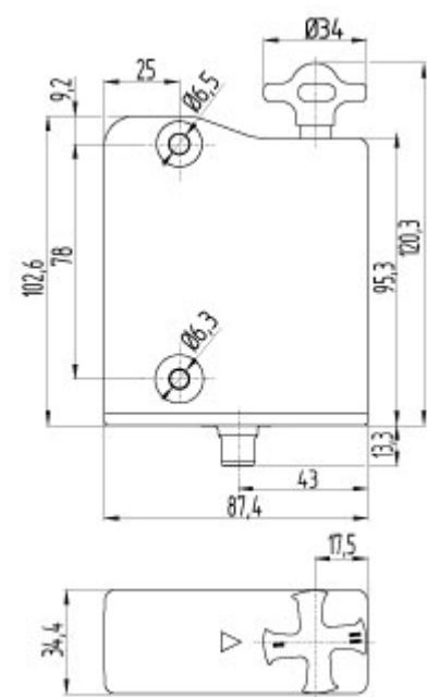
Dimensional drawing (basic component)
