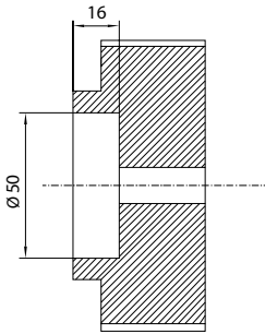
Turned groove Ø50x16 deep hub side
