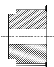
Synchronising pulley with 1 flange opposite the hub side
