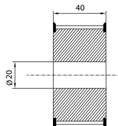
Synchronising pulley without hub
