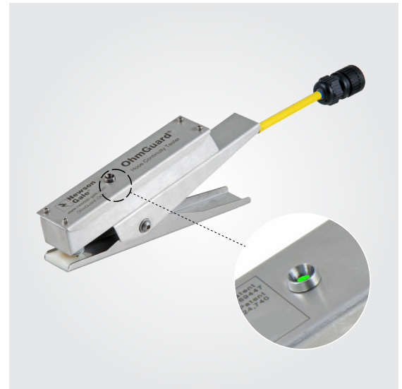
OhmGuard Intrinsically Safe Electrical Continuity Tester
