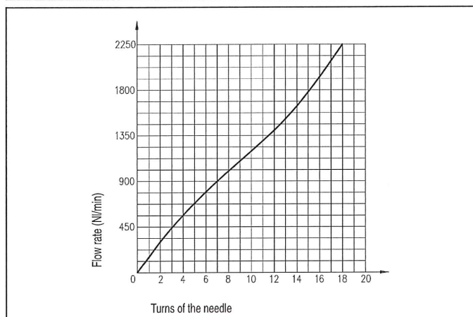
FLOW CHART at 6 bar - UR 2/25
