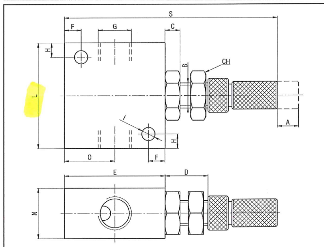
DIMENSIONS AND WEIGHTS URG - URF
