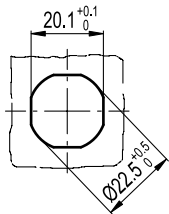
Drilling template
