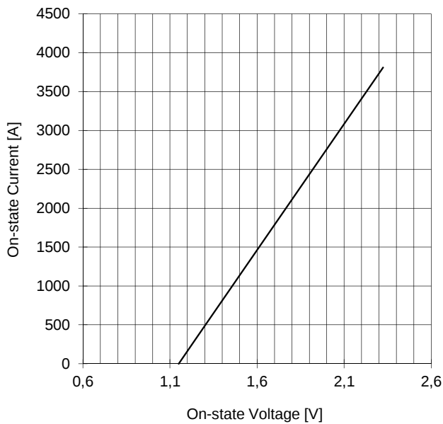
ON-STATE CHARACTERISTIC T_j = 125^\circ\text{C}
