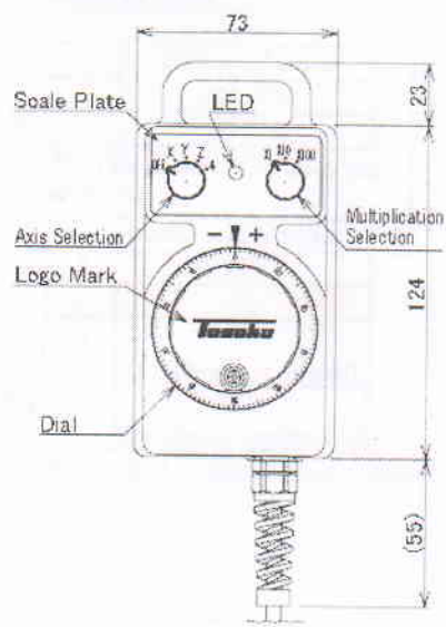
HC1 main unit with curl cord
