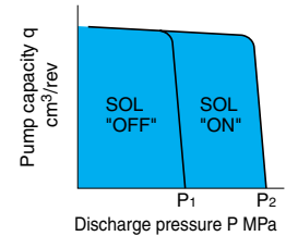
P-Q Characteristics
