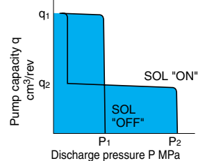
P-Q Characteristics
