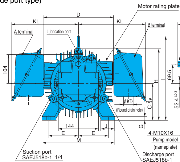
UPV-2A-35**-**-4-20 45 (side port type)
