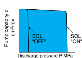
P-Q Characteristics
