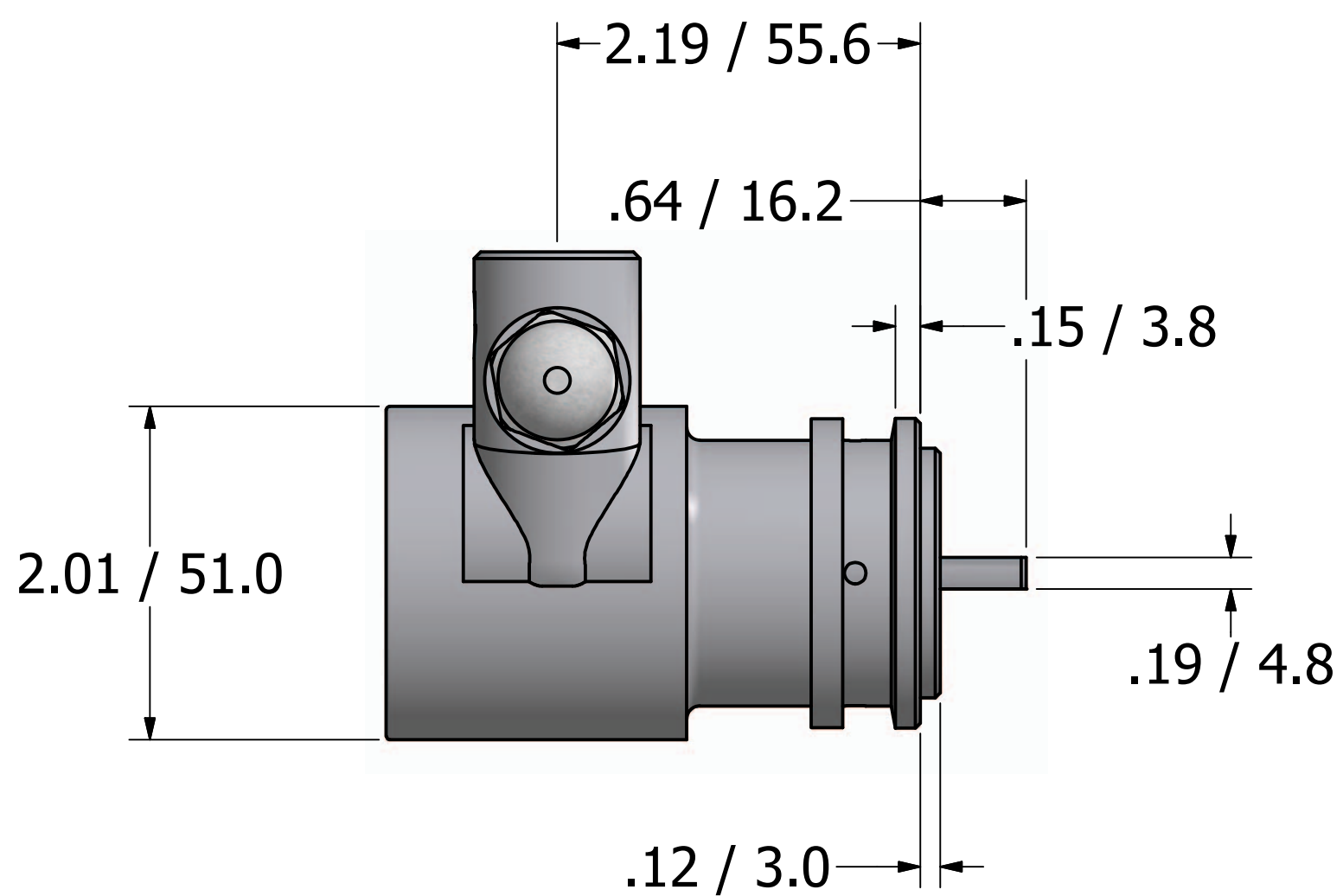
"A" Mounting
