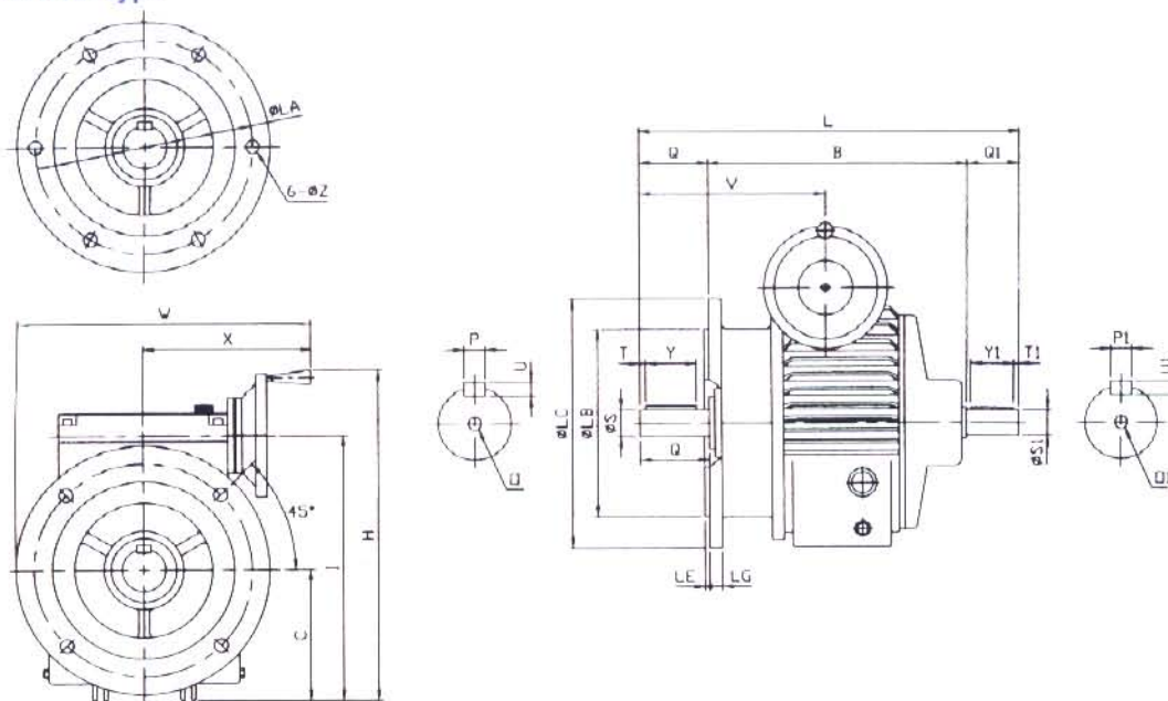
Two shaft vertical type
