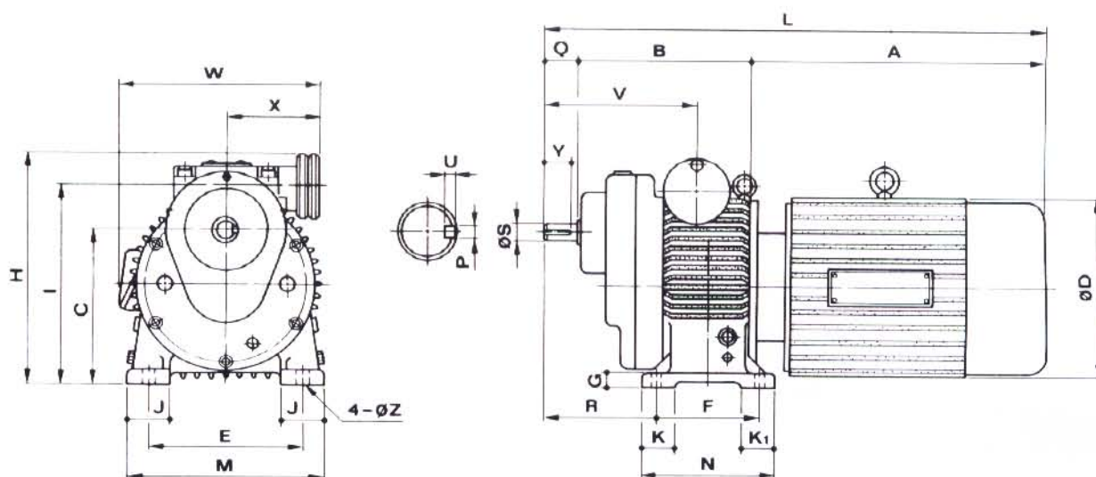
Horizontal type W/ " R " type reducer ( 1/2.5, 1/5 )
