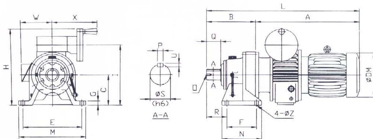
Horizontal type w/TRANSCYKO cycloidal speed reducer TDC-HM type ( 1/6 ~ 1/87 )
