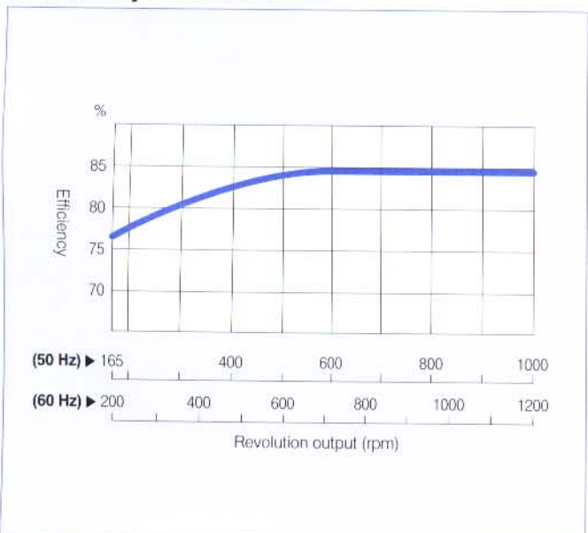
■ Efficiency-revolution curve
