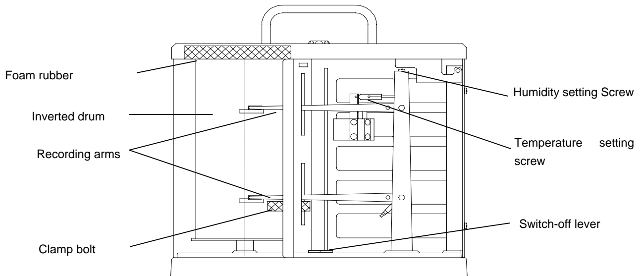
Figure 1: Hygro - Thermograph
