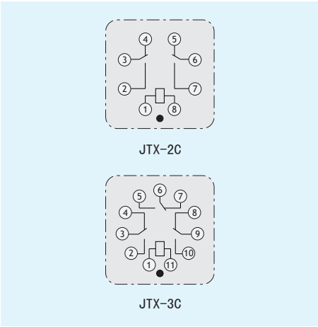
Internal connection (bottom view)
