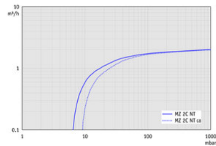
MZ 2C NT - Pumping speed graph at 60 Hz
