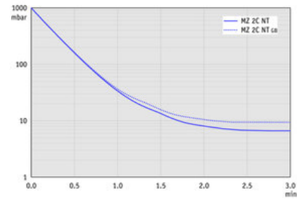
MZ 2C NT - Pump down graph at 60 Hz (10 l volume)
