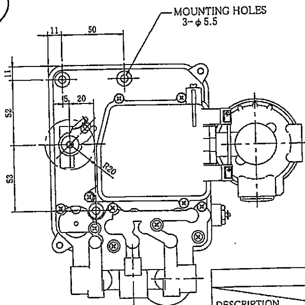
A VIEW
