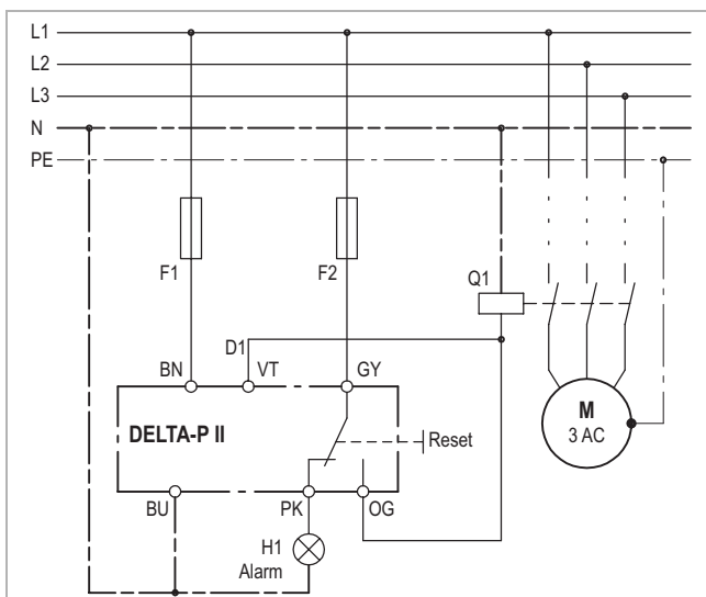
Wiring diagram
