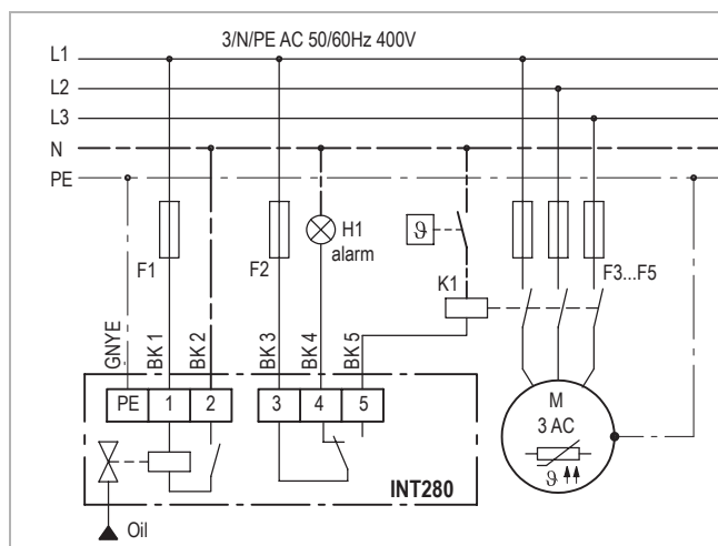
Wiring diagram
