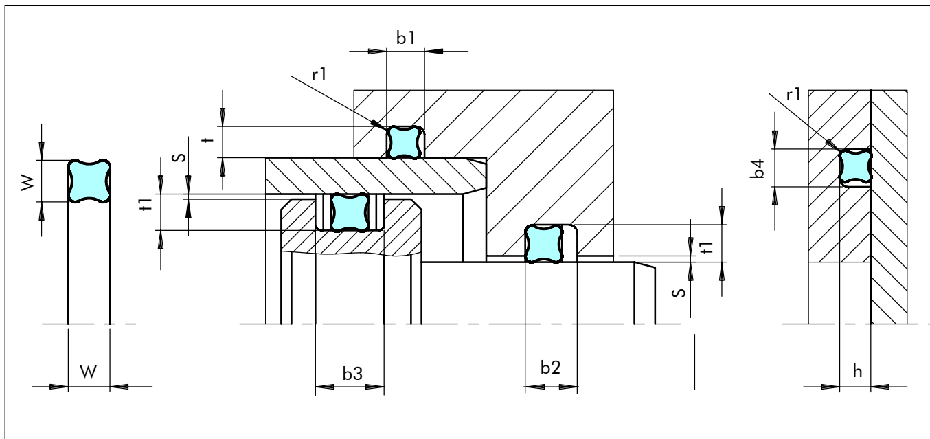
Figure 15 Installation drawing
