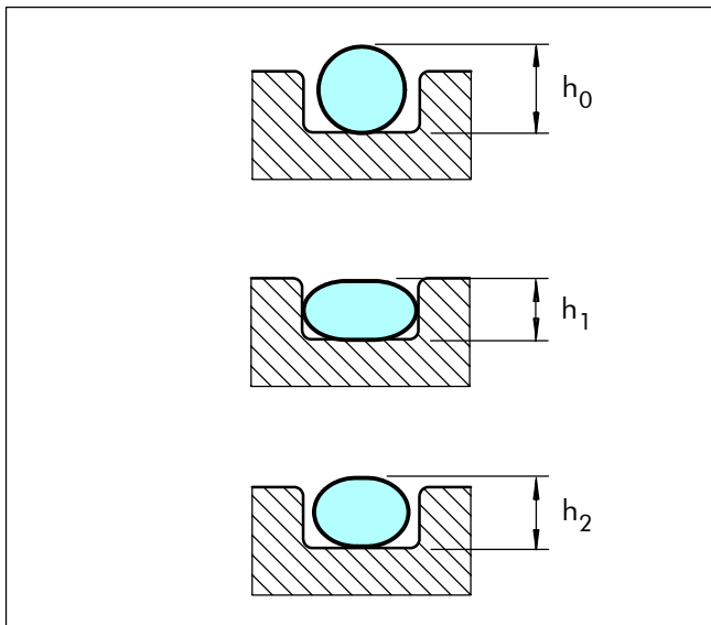
Figure 7 Illustration of the compression set
