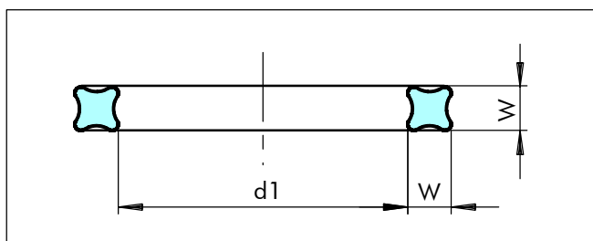
Figure16 QUAD-RING® Seal
