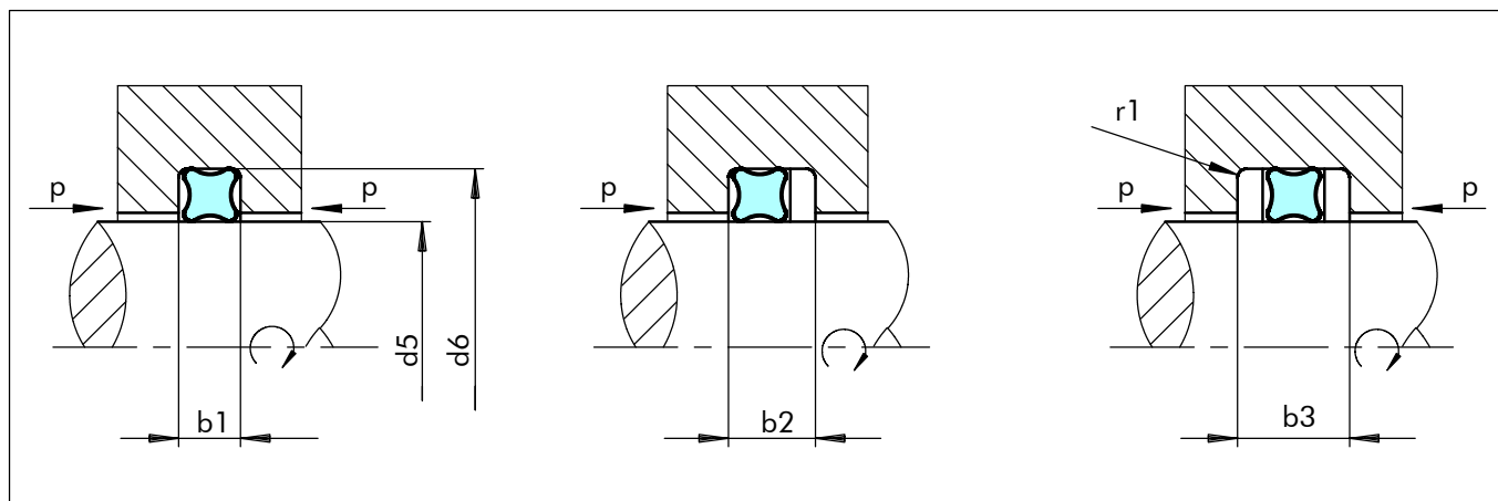
Figure19 Installation drawing
