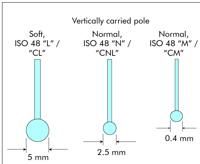
Figure 4 Indentor according to IRHD
