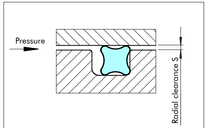
Figure 14 Radial clearance "S"
