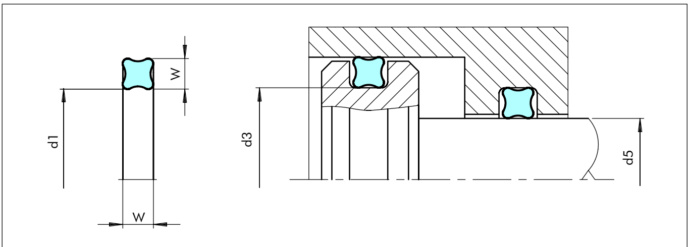
Figure 9 Radial installation, static and dynamic
