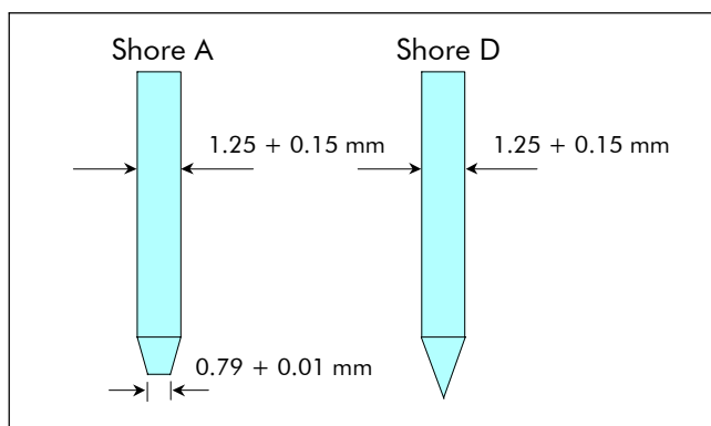
Figure 3 Indenter according to Shore A / D
