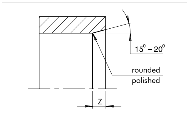
Figure 12 Lead-in chamfer for bores, tubes
