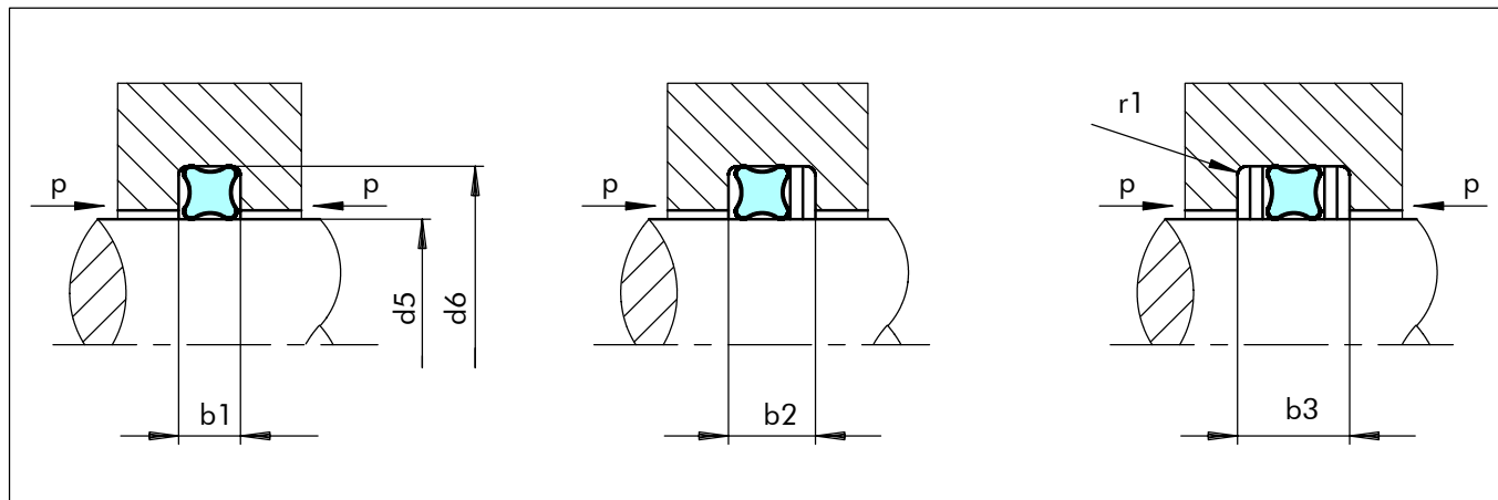
Figure18 Installation drawing
