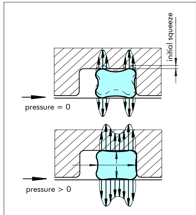
Figure 8 Sealing force with and without system pressure
