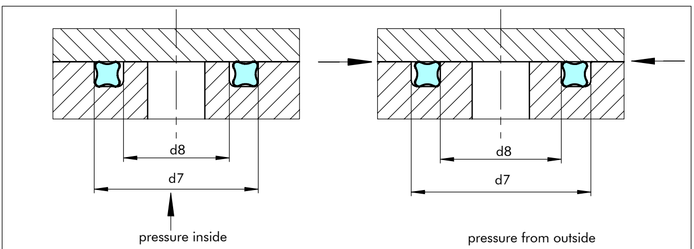
Figure 10 Axial installation, static
