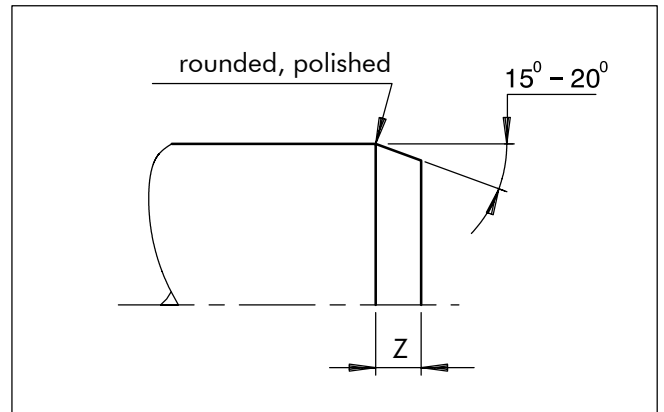
Figure 13 Lead-in chamfer for rods, shafts
