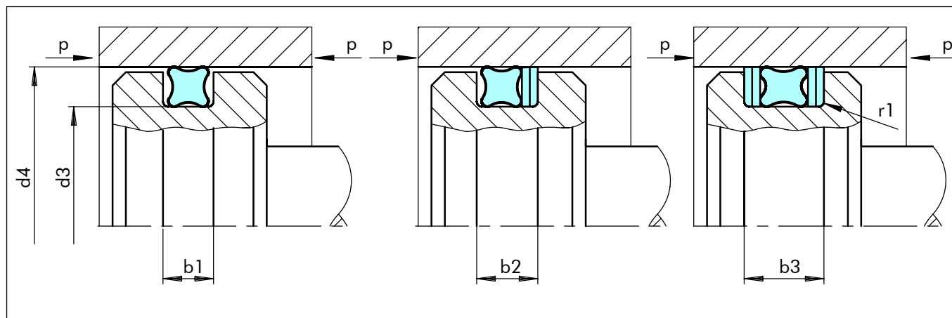
Figure17 Installation drawing
