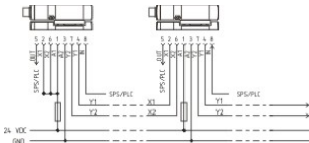
Wiring example
