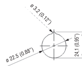
Ø 22mm (0,87") single-hole handle fixing
