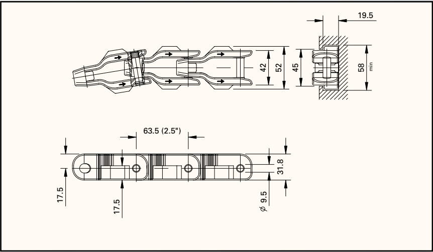
SIDEFLEX WITH TABS WITH HIGHER LINK
