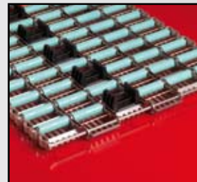
POSITRACK IN THE CENTER OF THE BELT OR 1.5" OFFSET, DEPENDING ON THE WIDTH
