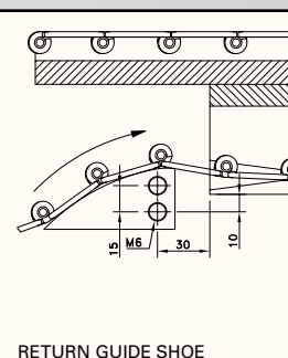
RETURN GUIDE SHOE
