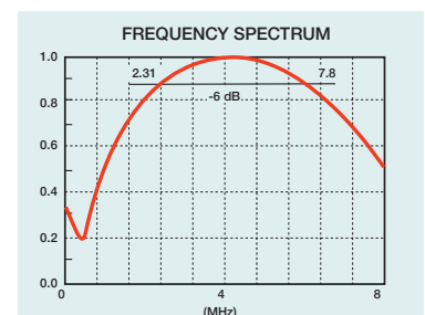
Signal waveform and frequency spectrum of CN4R-10
