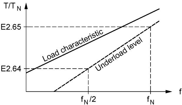
linear characteristic
