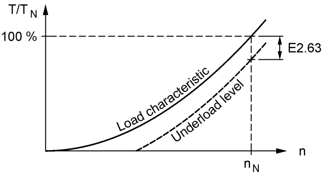
quadratic characteristic
